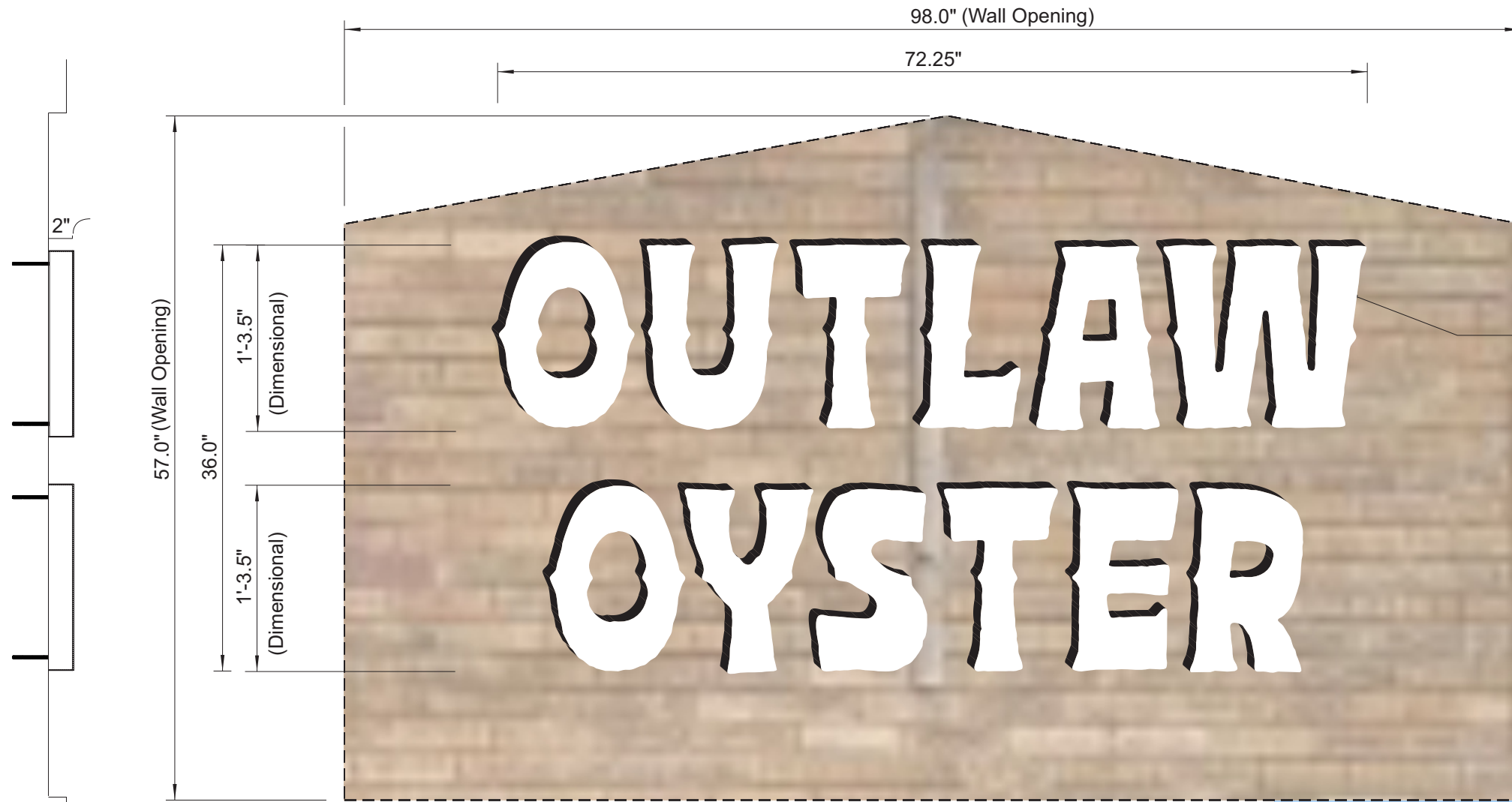
FRONT VIEW 1" = 1' - 0" Scale
