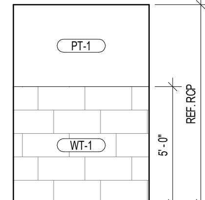
21 JANITOR CLOSET 1/4" = 1'-0"
