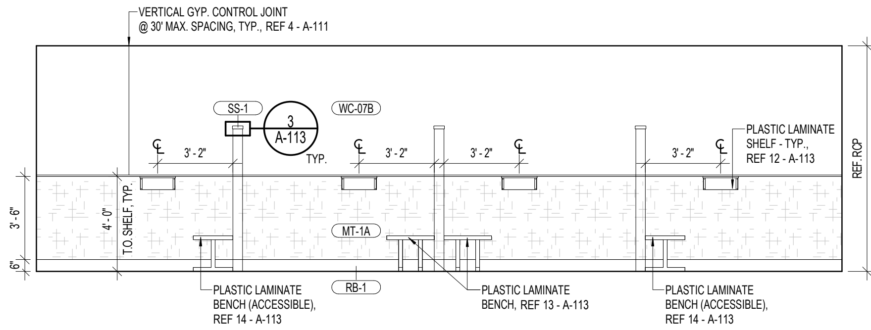
2 HYDROMASSAGE 1/4" = 1'-0"
