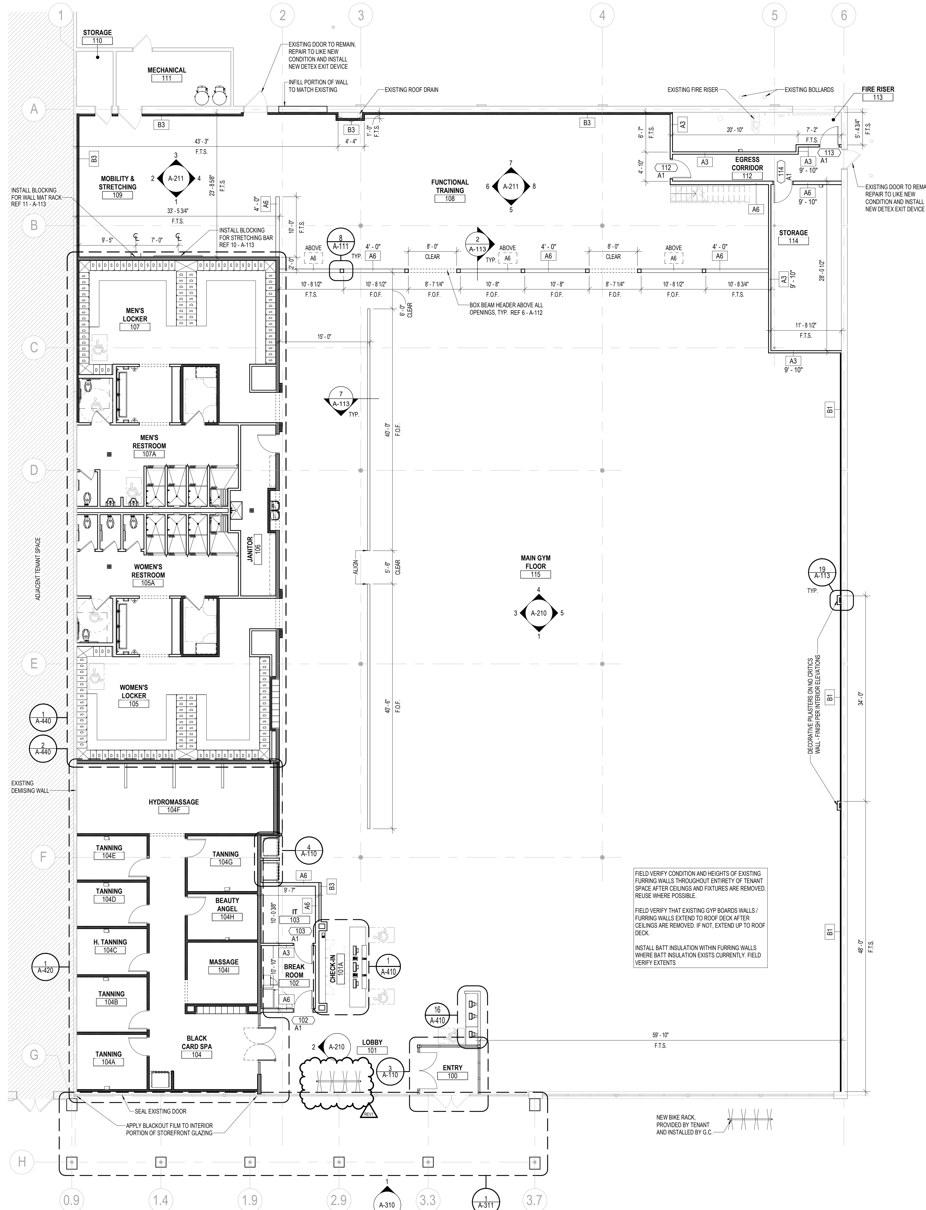
1 CONSTRUCTION PLAN 1/8" = 1'-0"
