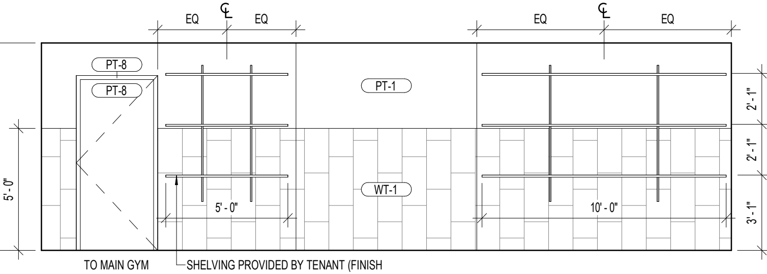
24 JANITOR CLOSET 1/4" = 1'-0"
