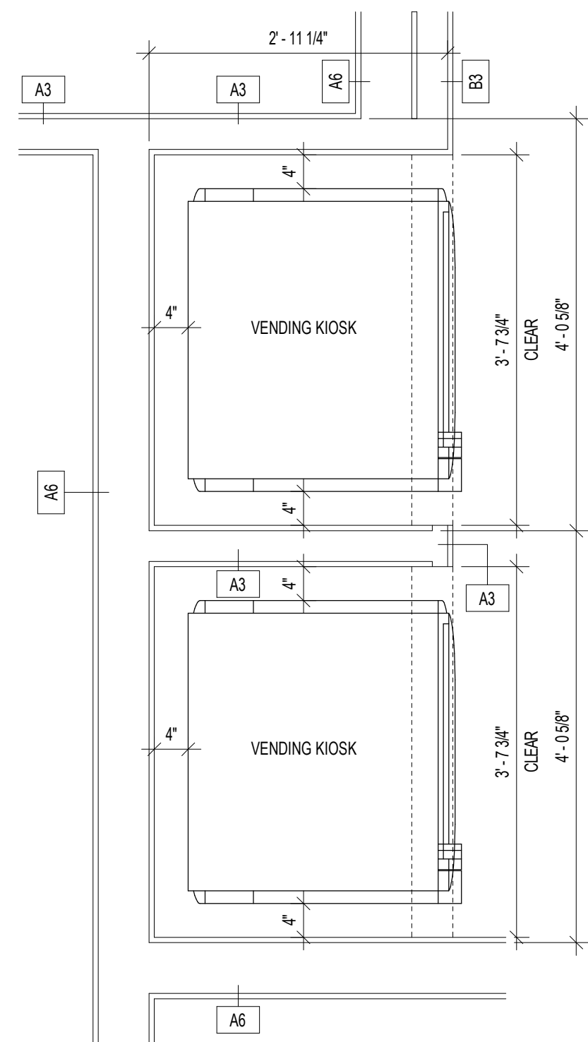
4 ENLARGED PLAN - VENDING KIOSKS 3/4" = 1'-0"
