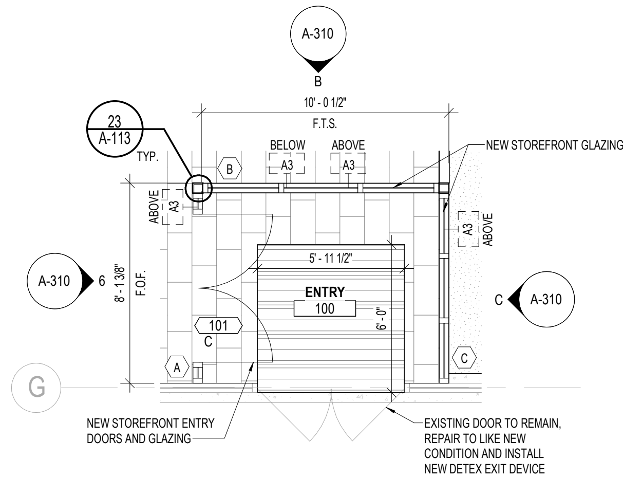
3 ENLARGED PLAN - VESTIBULE 1/4" = 1'-0"
