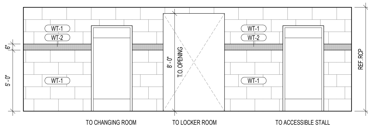
13 RESTROOM / SHOWERS (S.O.H.) 1/4" = 1'-0"
