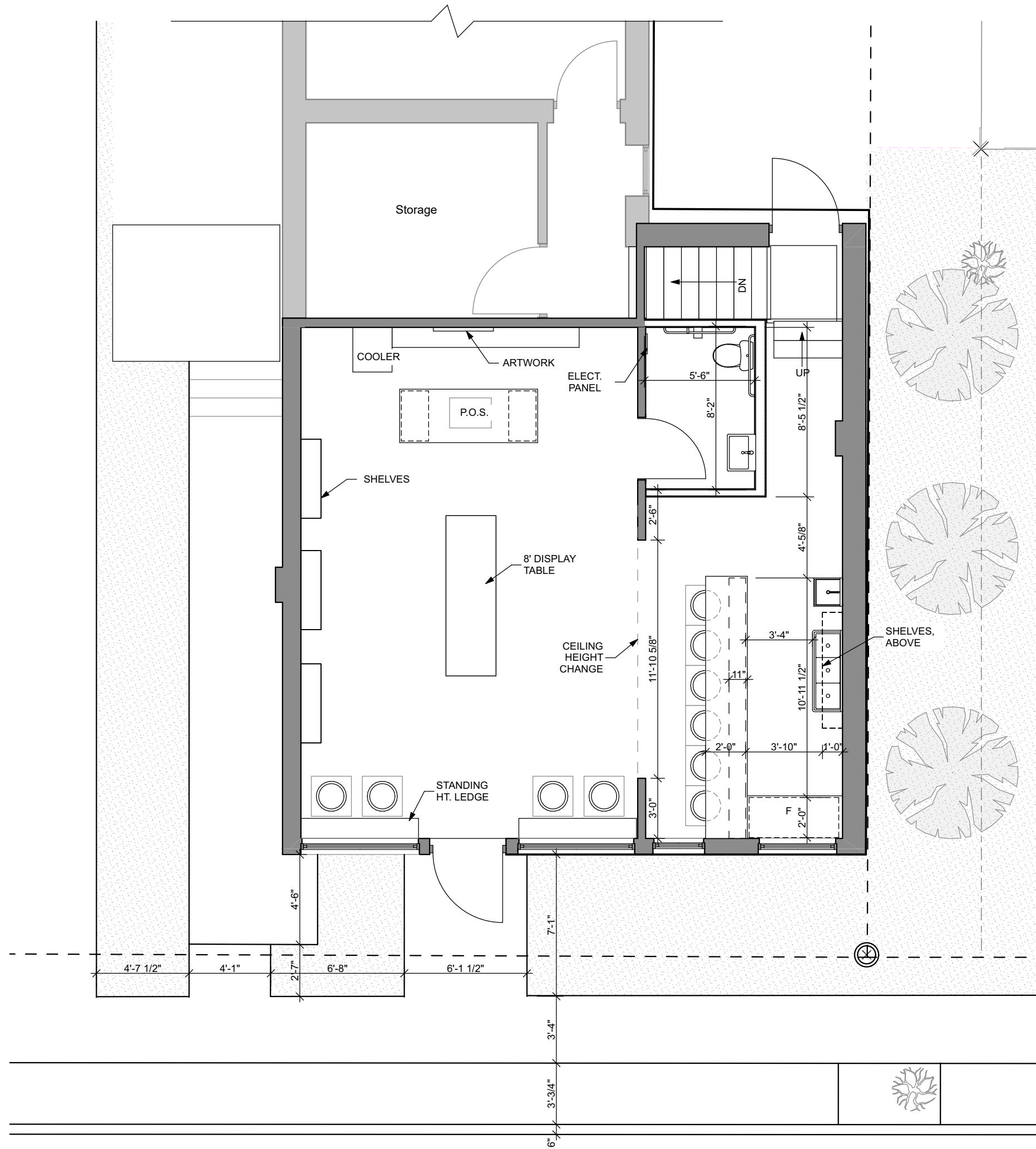
1 A101A GROUND LEVEL SCALE: 3/16" = 1'-0"
