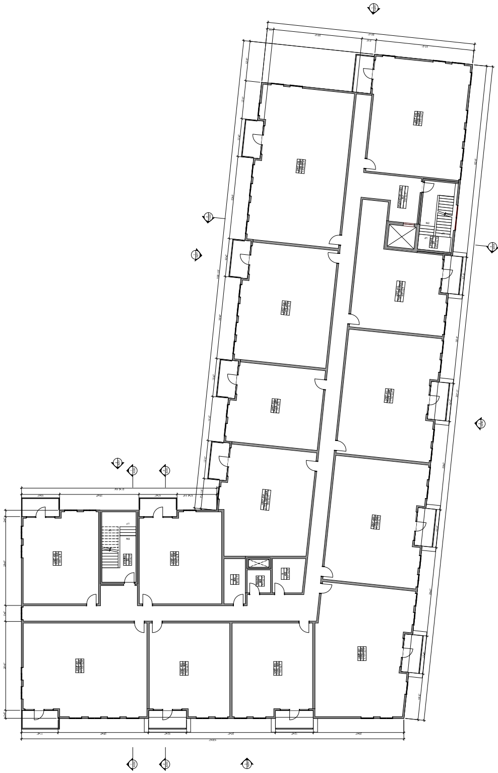
FOURTH FLOOR SCALE: 1/8" = 1'-0"
