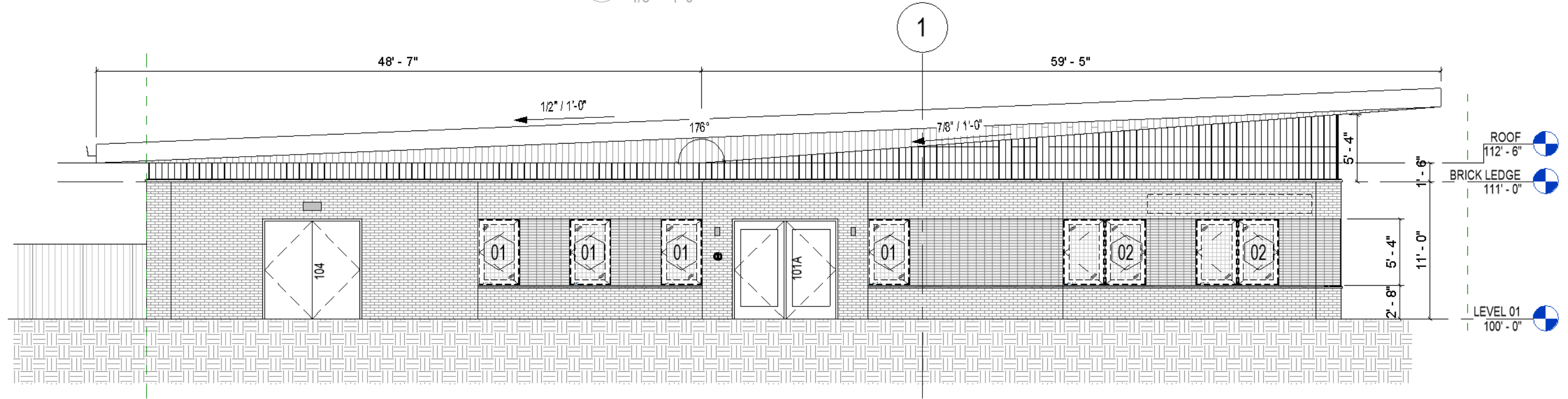
SOUTH ELEVATION
