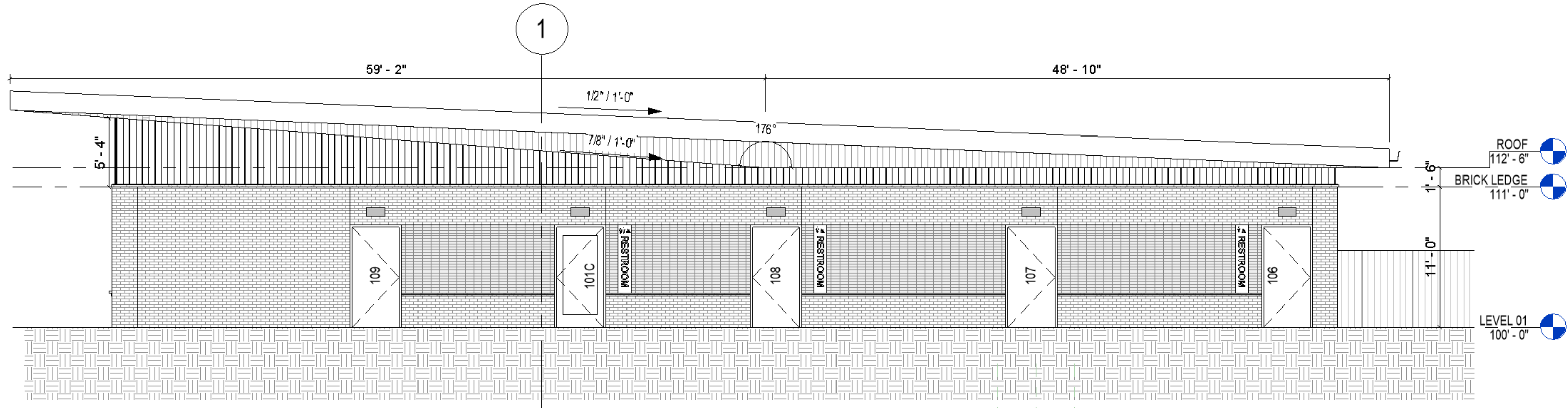
SOUTH ELEVATION
