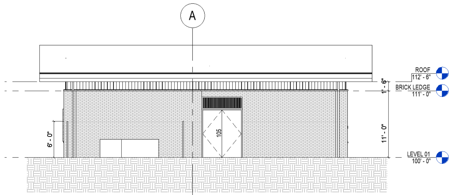
EAST ELEVATION
